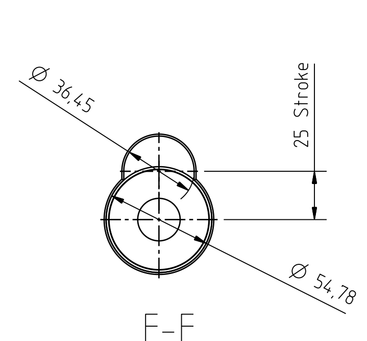
F-F
